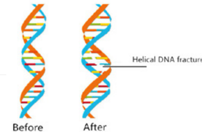
DNA HELIX
